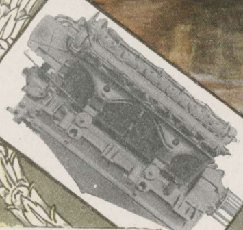
Side View of the 350 B.H.P. 12 Cylinder Sunbeam Coatalen Aircraft Engine.
