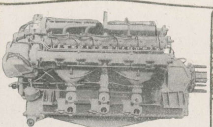
Side View of the 475 B.H.P. 18 Cylinder Sunbeam-Coatalen Aircraft Engine.
